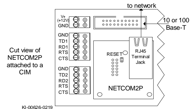
Figure 2 - NETCOM2P/CIM Secondary Connection
