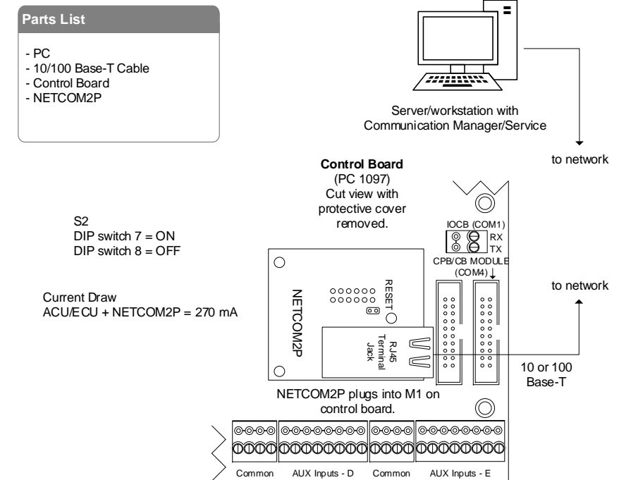
Figure 2 - NETCOM2P/CIM Secondary Connection
